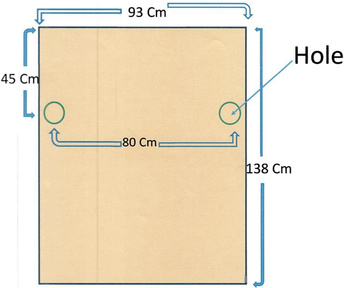
Dimension of Electronic Metering pump Base
